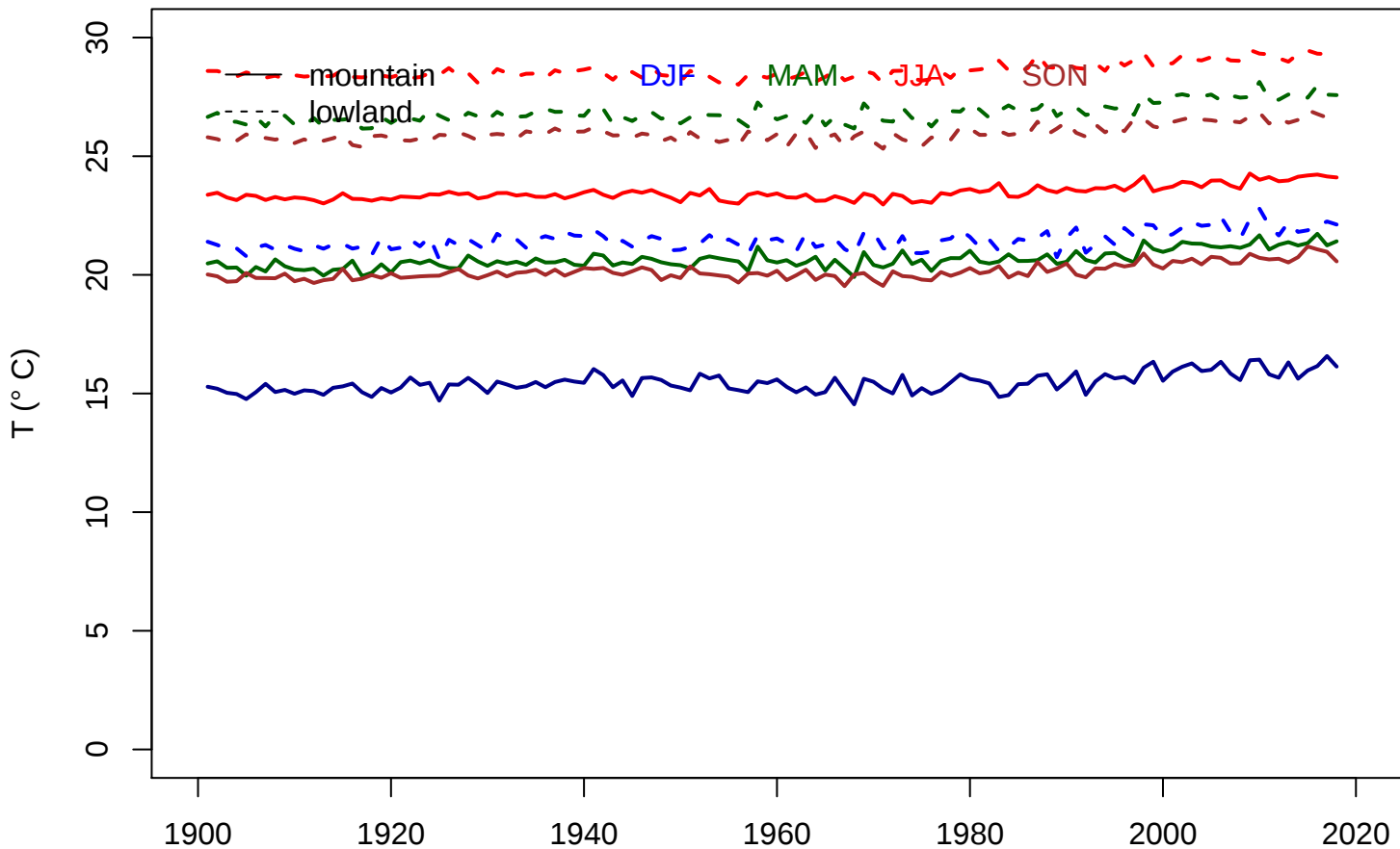
Temperature timeseries for CRU 0–30N
